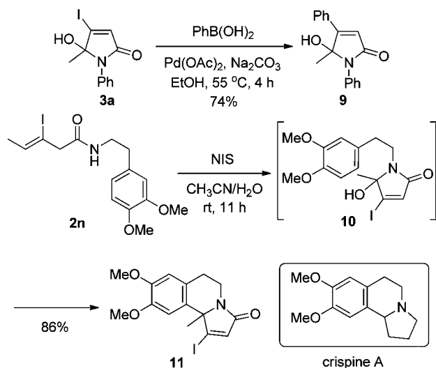
Scheme 2. Application of Vinyl Iodo Amides
