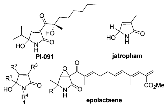
Figure 1. Examples of pyrrolidinone-containing natural products.
