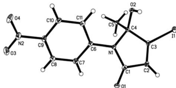
Figure 2. X-ray structure of 3e .
