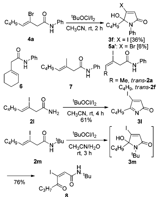
Scheme 1. Miscellaneous Alkenyl Amide Reactions
