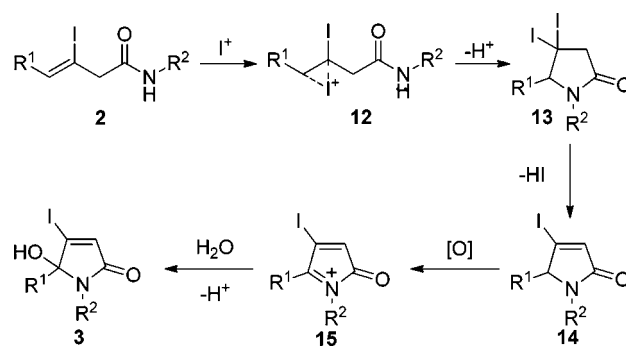
Scheme 3. Proposed Mechanism for Formation of 3
